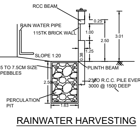
RAINWATER HARVESTING
