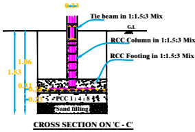
CROSS SECTION ON C - C
