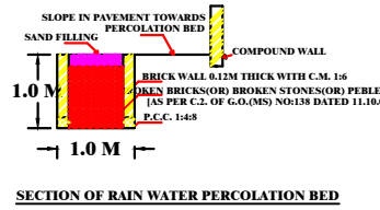
SECTION OF RAIN WATER PERCOLATION BED
