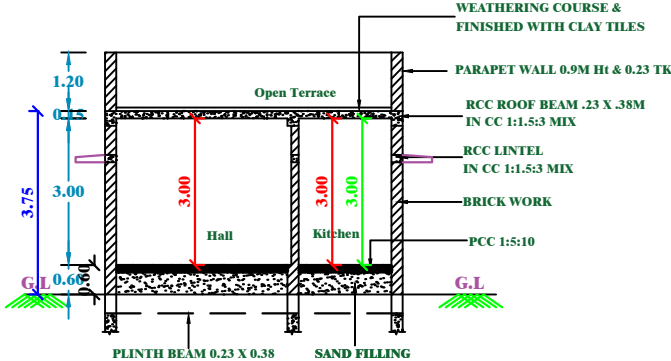
SECTION-XX
