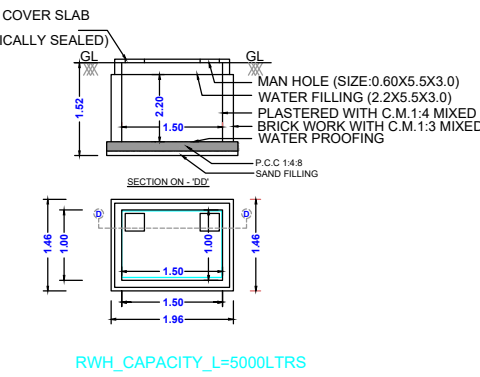
DETAILS OF COLLECTION SUMP FOR RAIN PLAN
