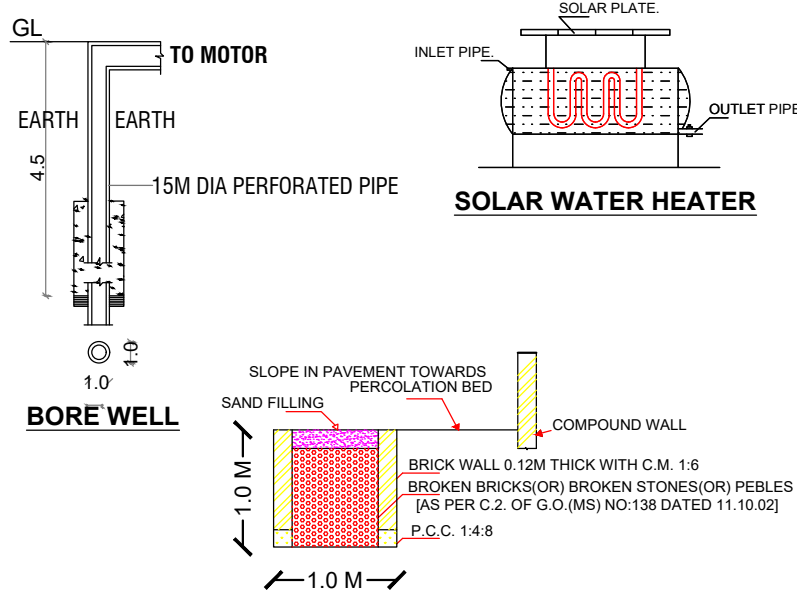
SECTION OF RAIN WATER PERCOLATION BED
