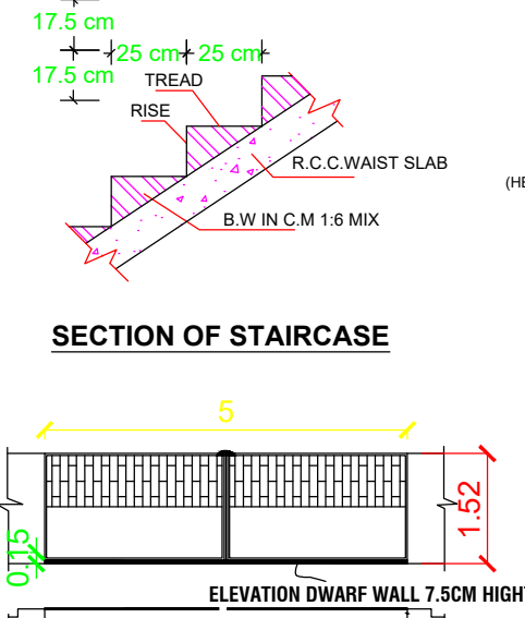
GATE ELEVATION
