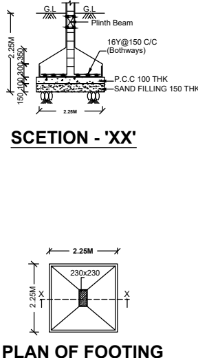
PLAN OF FOOTING
