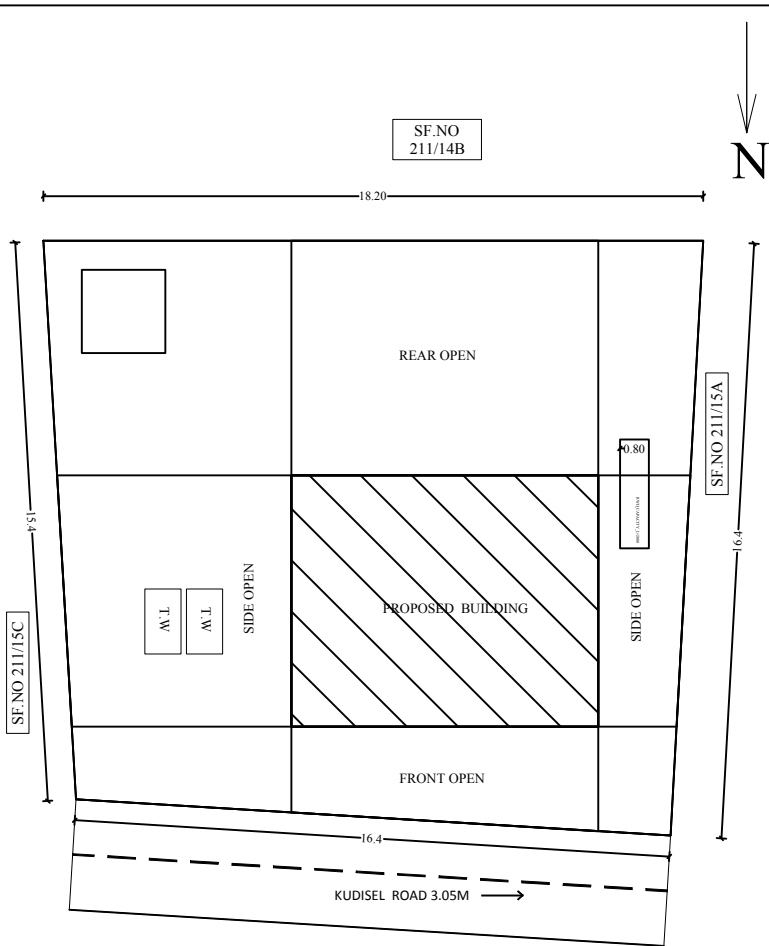
SITE PLAN
