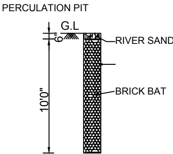
PERCOLATION PIT
