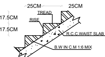
SECTION OF STAIRCASE
