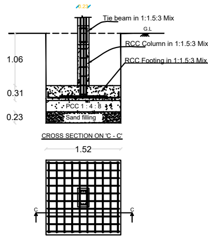
COLOUMN FOUNDATION
