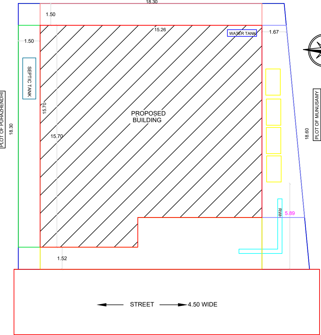
SITE PLAN
