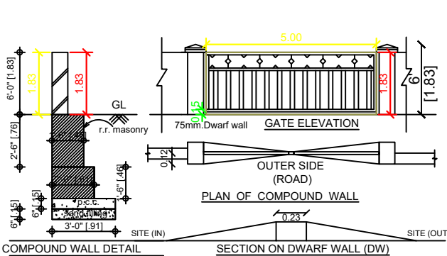
DETAILS OF COMPOUND WALL
