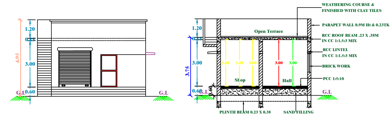
FRONT ELEVATION
