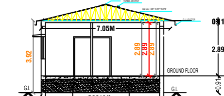
SECTION 'X-X'
