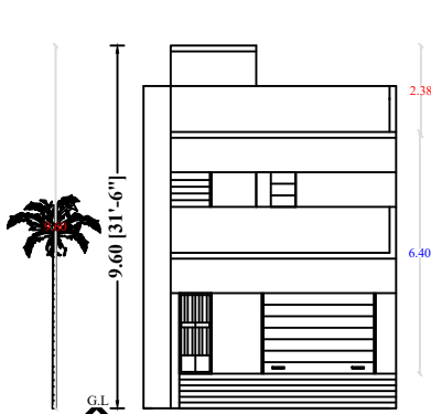
FRONT ELEVATION
