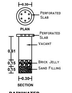
RAINWATER PERCOLATION PIT @ 3M INTERVAL
