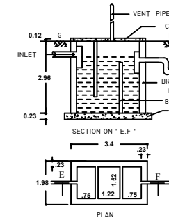
TOILET / SEPTIC TANK DETAILS ( NOT TO SCALE )
