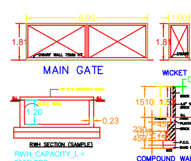
MAIN GATE WICKET GATE DETAILS ( NOT TO SCALE )
