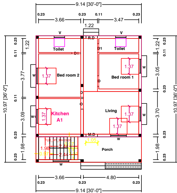
FLOOR 0 (GROUND) PLAN ( FACING EAST )
