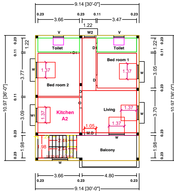
FLOOR 1 ( FIRST ) PLAN ( FACING EAST )
