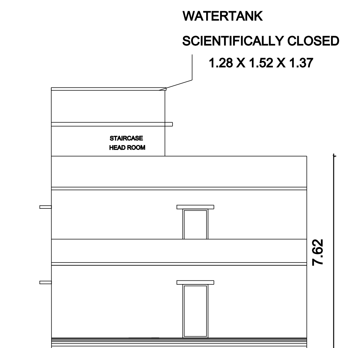
FRONT ELEVATION.
