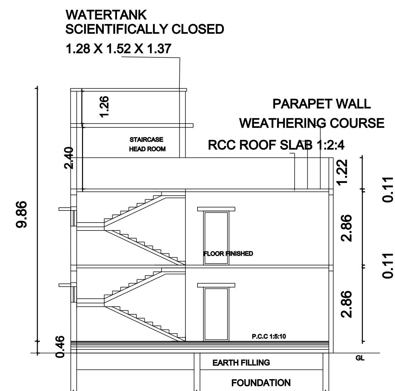
SECTION "A-B"
