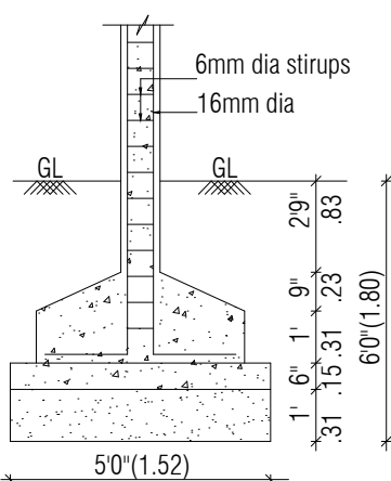
FOUNDATION DETAIL
