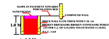
SECTION OF RAIN WATER PERCOLATION BED
