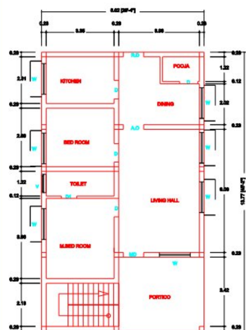
GROUND FLOOR PLAN (SOUTH FACING)
