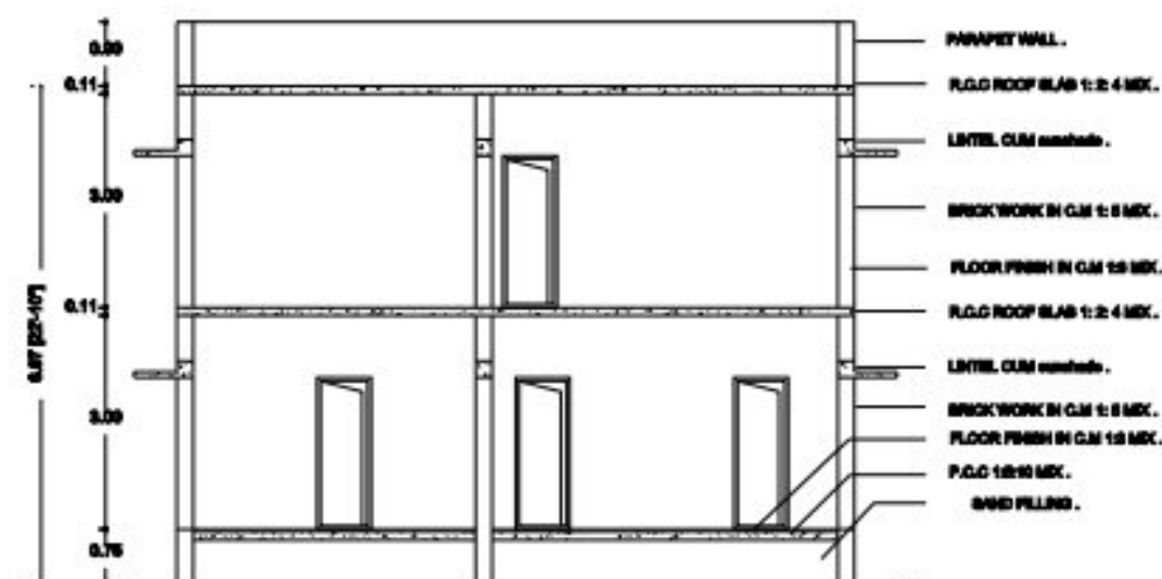
CROSS SECTION ON 'AB'
