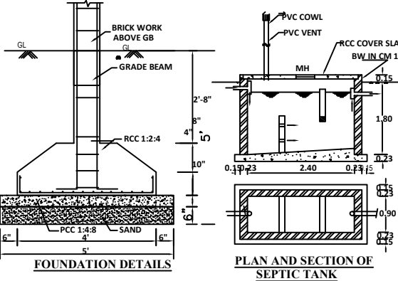
FOUNDATION DETAILS
