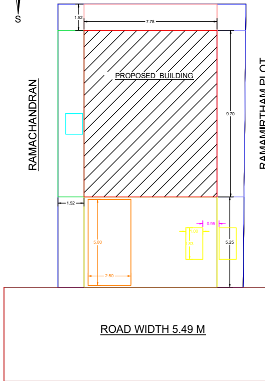
SITE PLAN 1:100 SCALE BALAKRISHNAN SITE
