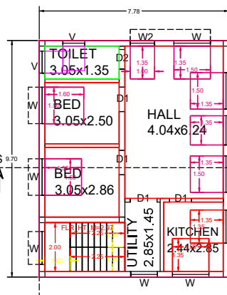
PROPOSED FIRST FLOOR
