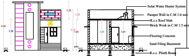
FRONT ELEVATION
