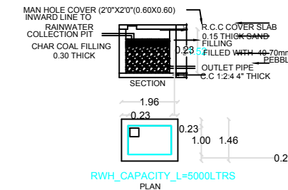
DETAIL OF RAINWATER HARVESTING
