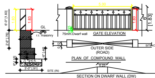
DETAIL OF COMPOUND WALL
