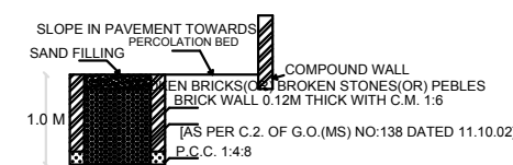
SECTION OF RAIN WATER PERCOLATION BED
