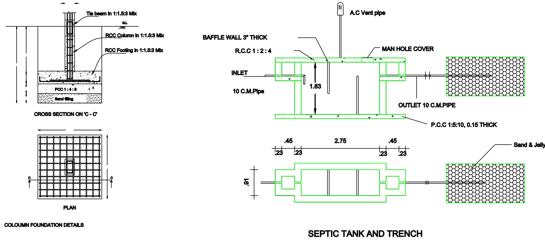
SEPTIC TANK AND TRENCH
