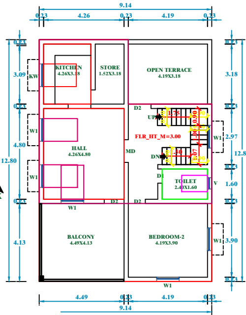
3D EXTENSION OF GROUND FLOOR PLAN
