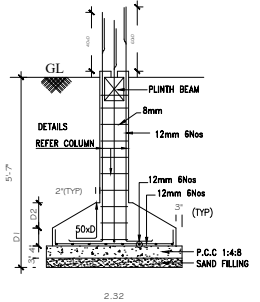
FOUNDATION DETAILS SCALE : 1:50.
