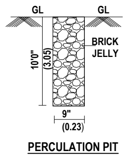
PERCOLATION PIT
