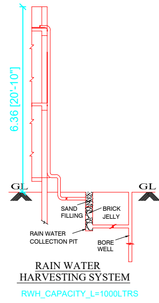
RAIN WATER HARVESTING SYSTEM RW.H_CAPACITY_L=1000L.TRS
