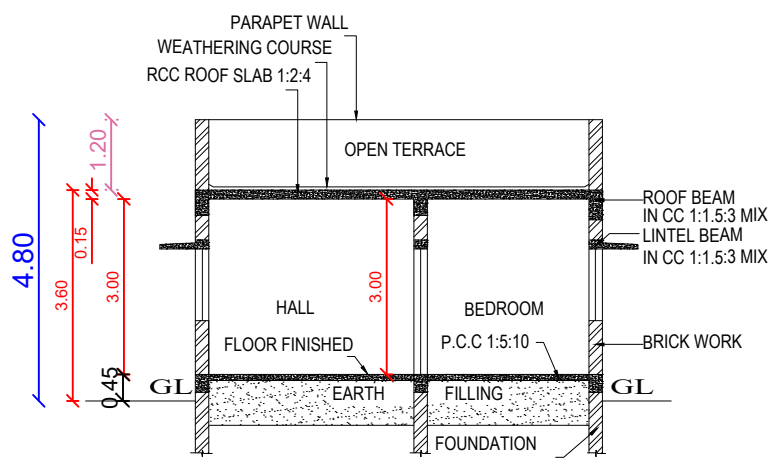
SECTION "A-B"
