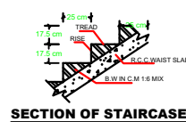
SECTION OF STAIRCASE
