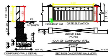
DEATILS OF COMPOUND WALL
