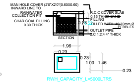
DEATILS OF RAINWATER HARVESTING
