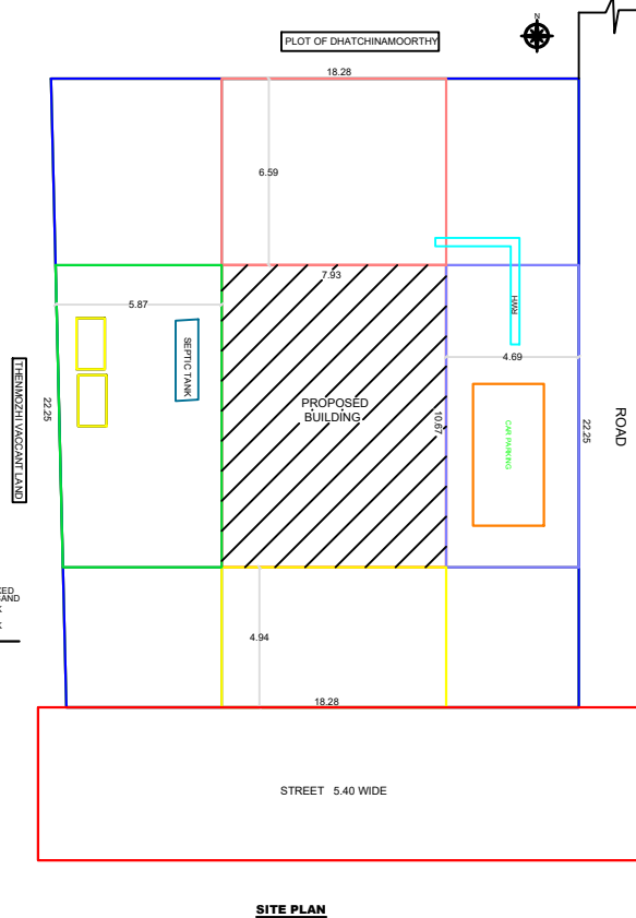
SITE PLAN
