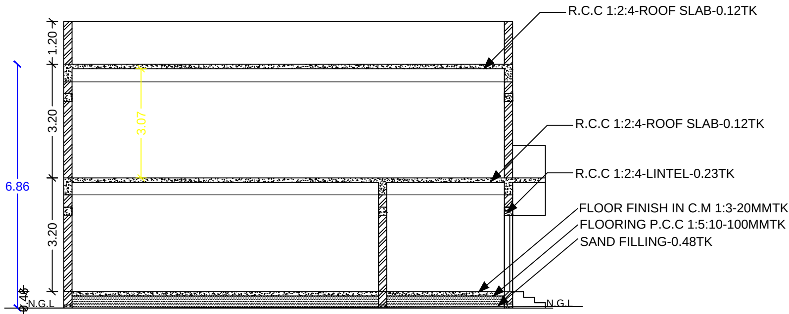
CROSS SECTION "SS"
