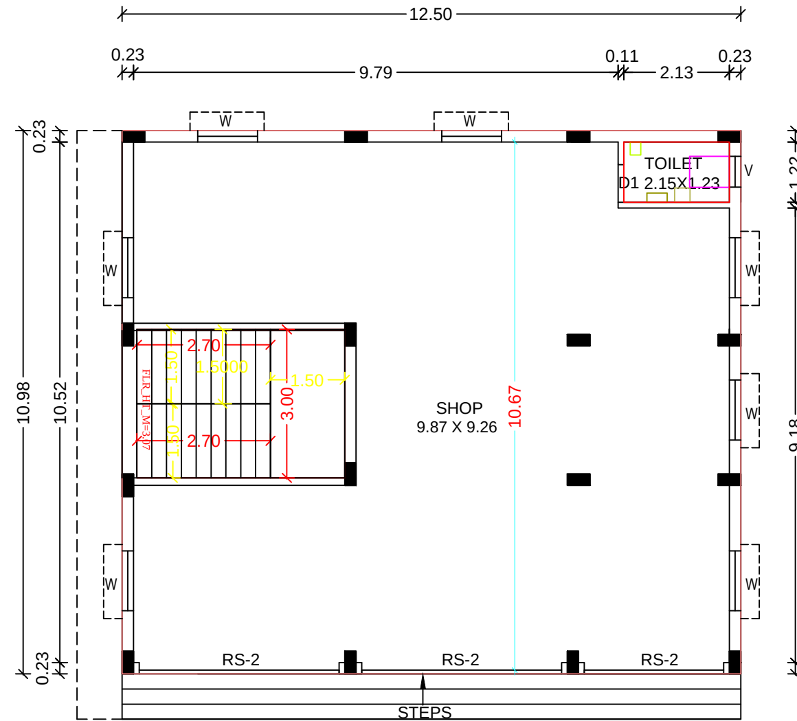
GROUND FLOOR PLAN (EXISTING APPROVED)
