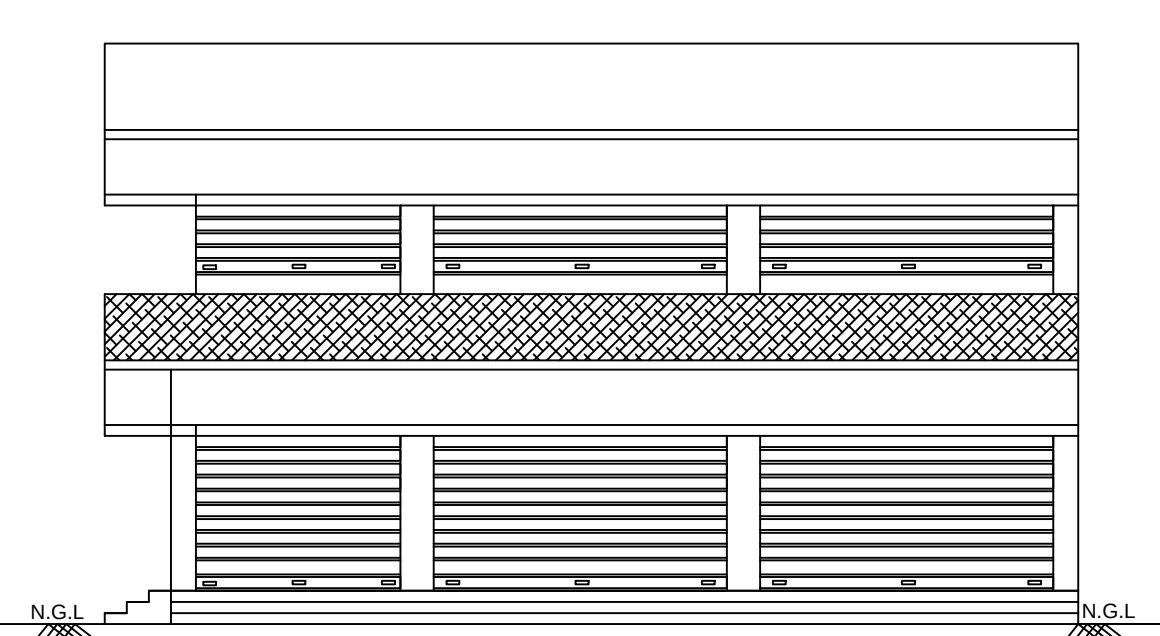
FRONT ELEVATION
