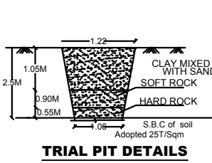
TRIAL PIT DETAILS
