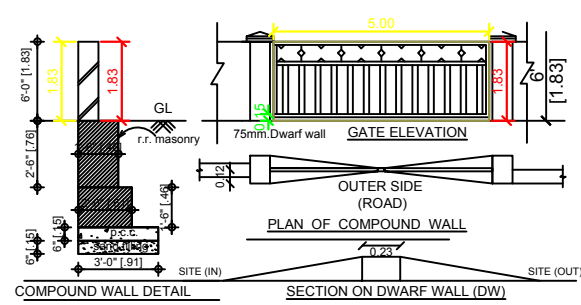
DETAILS OF COMPOUND WALL
