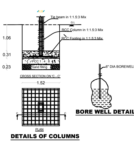
DETAILS OF COLUMNS
