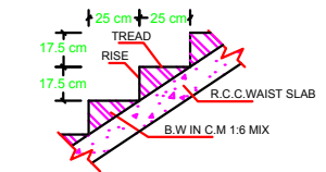
SECTION OF STAIRCASE
