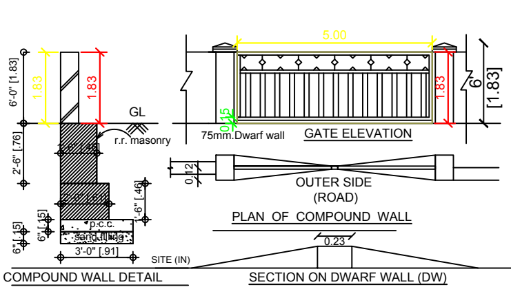
DETAILS OF COMPOUND WALL
