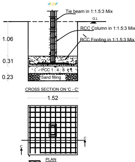
COLOUMN FOUNDATION
