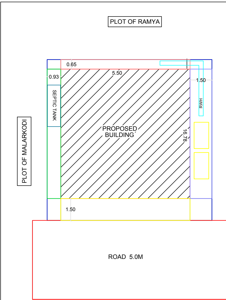
SITE PLAN
