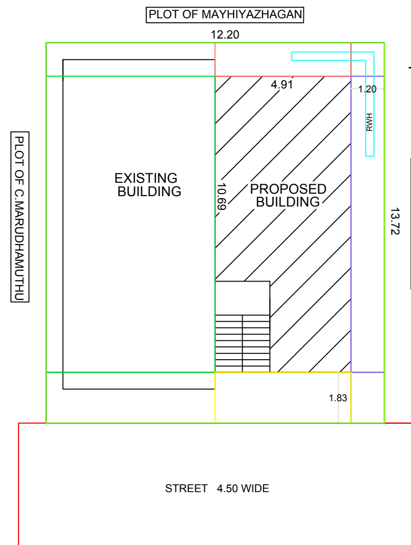
SITE PLAN
