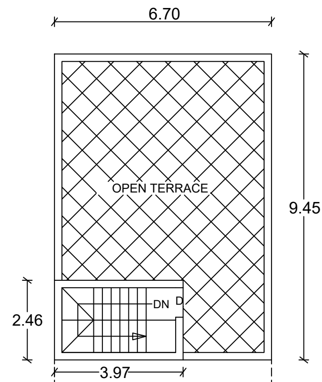
TERRACE & HEAD ROOM PLAN
