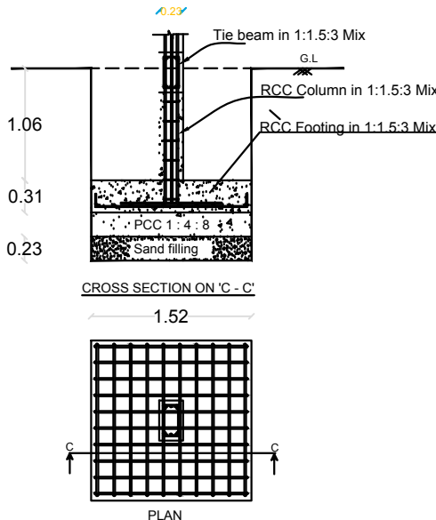
COLOUMN FOUNDATION
