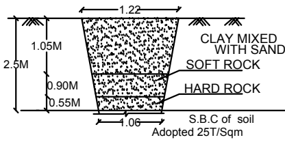
TRIAL PIT DETAILS
