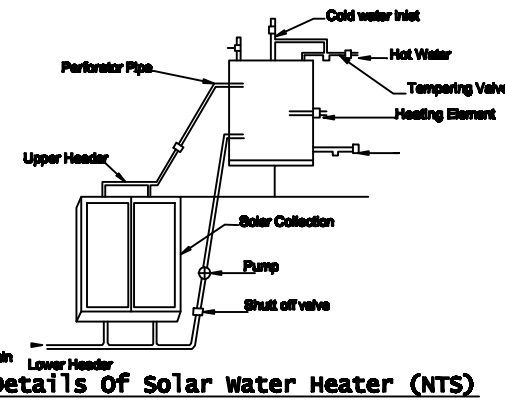
Details of Solar Water Heater (NTS)
