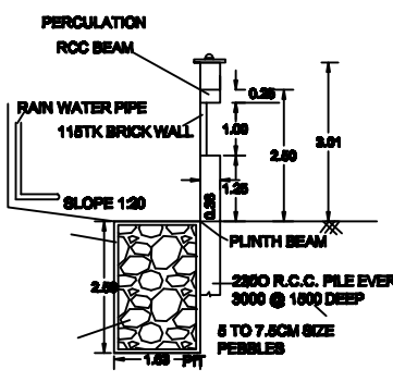
RAINWATER HARVESTING
