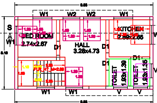
FIRST FLOOR (PROPOSED)
