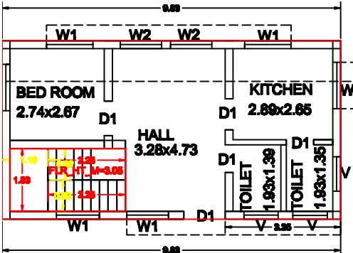
GROUND FLOOR(EXISTING)
