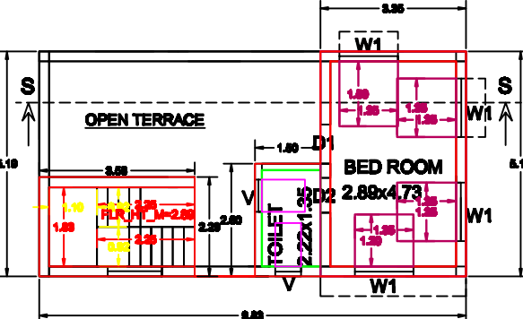
SECOND FLOOR(PROPOSED)
