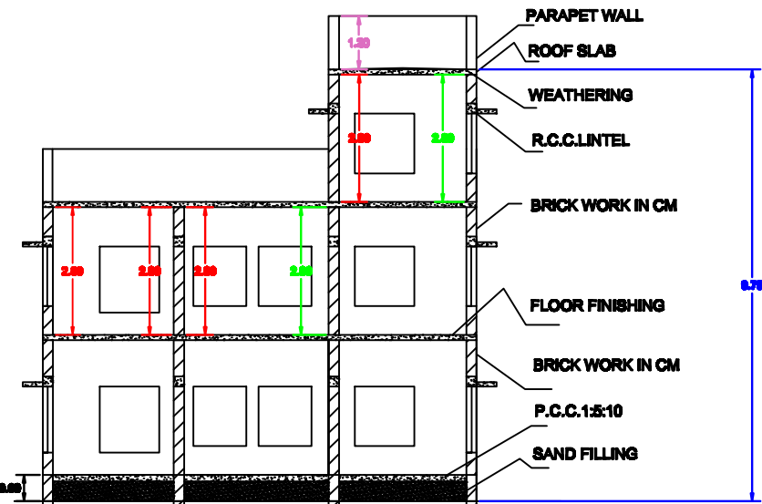
SECTION ON SS
