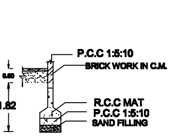
FOUNDATION DETAILS
