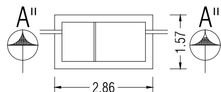
SEC. OF SEPTIC TANK "AA"
