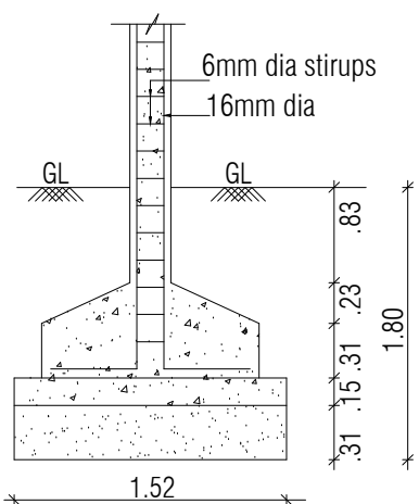
FOUNDATION DETAIL
