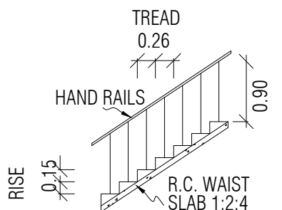
STAIRCASE DETAILS
