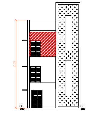
FRONT ELEVATION
