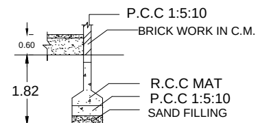
FOUNDATION DETAILS
