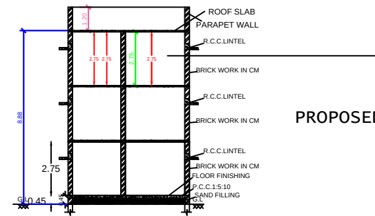
SECTION ON SS
