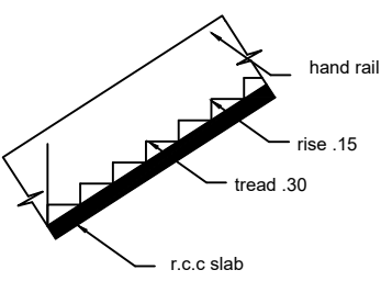
STAIR
