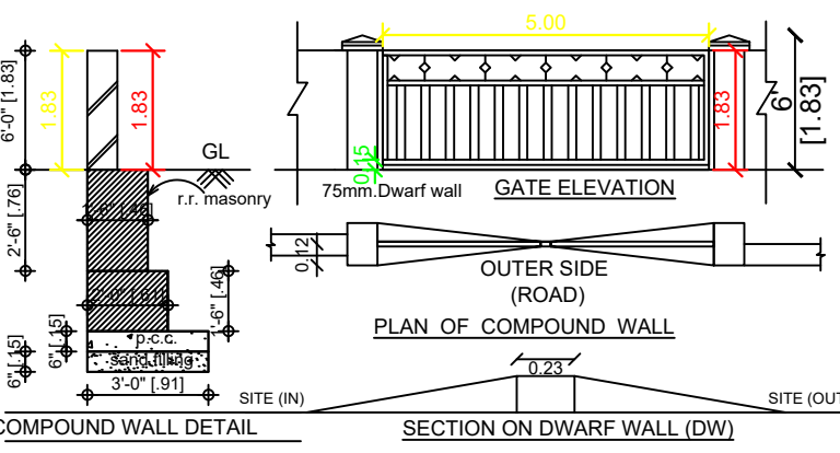
COMPOUND WALL DETAIL
