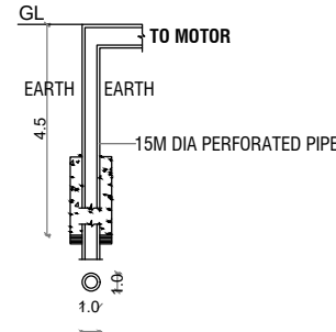
BORE WELL
