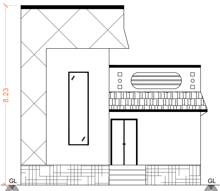
FRONT ELEVATION
