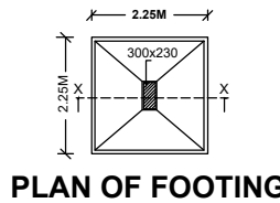
PLAN OF FOOTING
