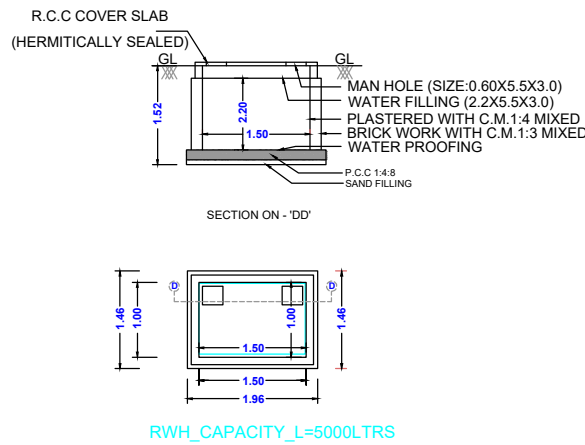
DETAILS OF COLLECTION SUMP FOR RAIN PLAN
