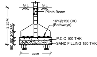
SECTION - "XX"
