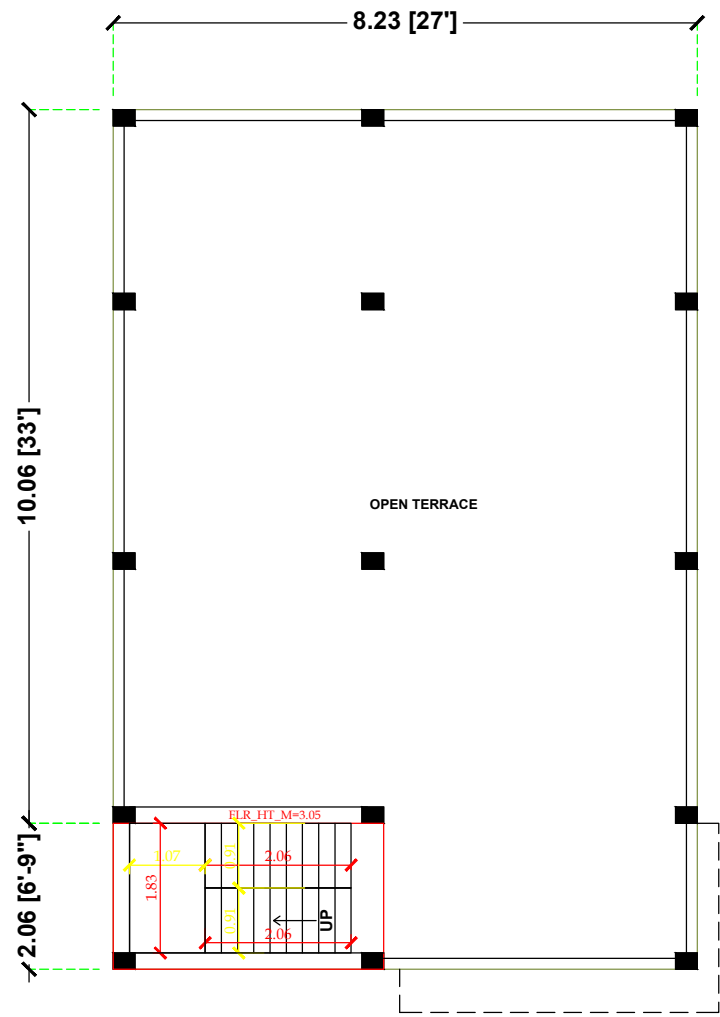
TERRACE PLAN
