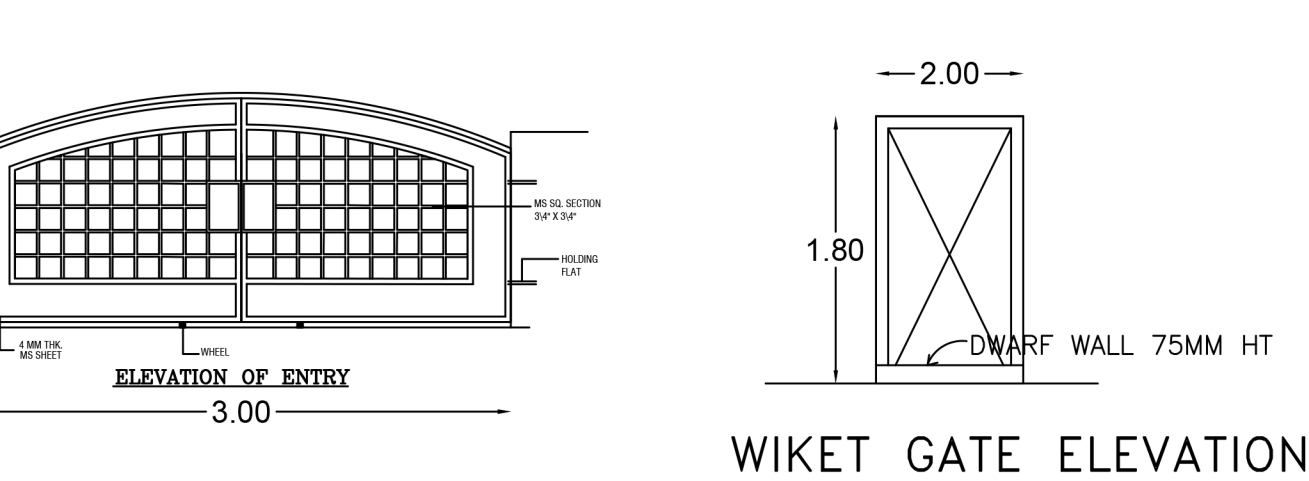
WIKET GATE ELEVATION
