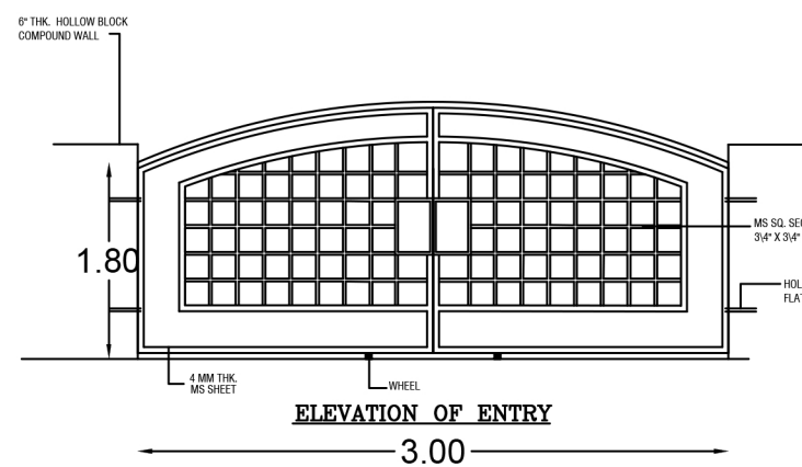
ELEVATION OF ENTRY
