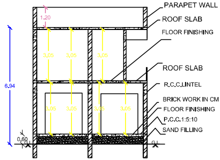
SECTION ON SS
