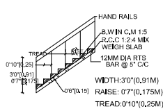
SECTION ON SS
