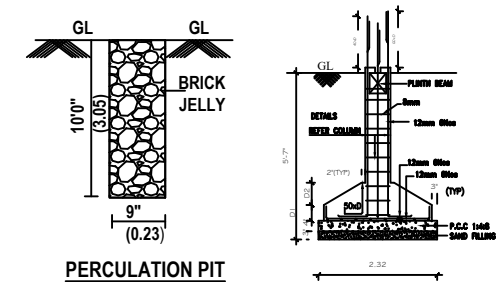
FOUNDATION DETAILS SCALE : 1:50.
