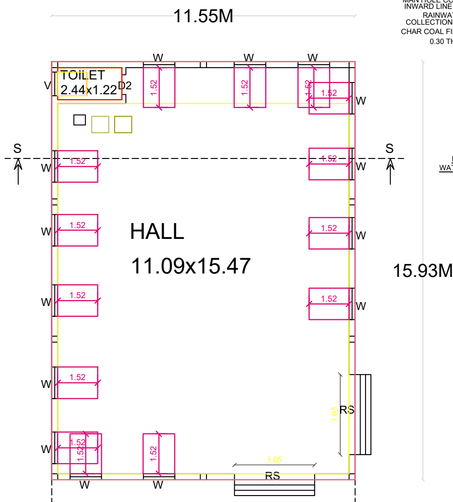
GROUND FLOOR
