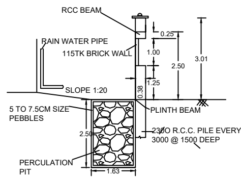
RAINWATER HARVESTING
