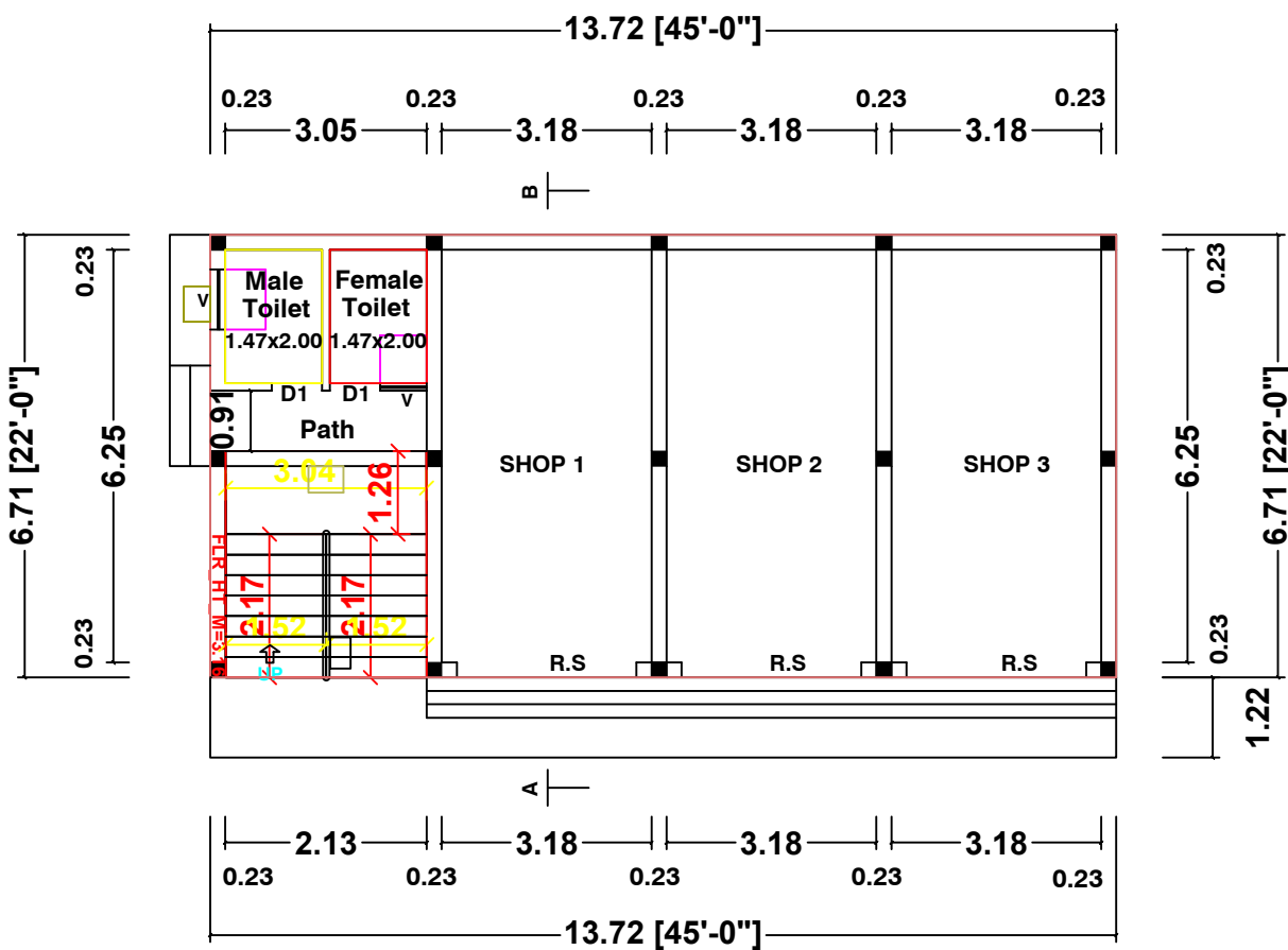
FLOOR-0 (GROUND) PLAN ( FACING SOUTH )
