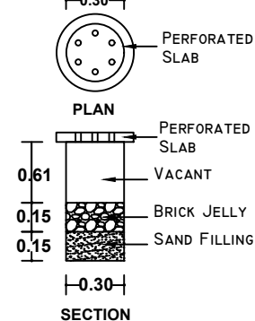
RAINWATER PERCOLATION PIT @ 3M INTERVAL
