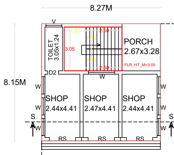
EXISTING GROUND FLOOR
