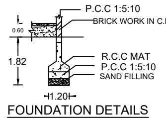
FOUNDATION DETAILS
