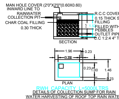
RAIN WATER HARVESTING OF ROOF TOP RAIN WATER
