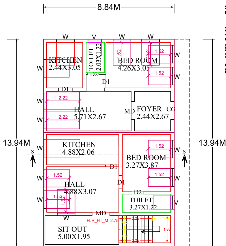
PROPOSED SECOND FLOOR
