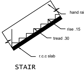
STAIR
