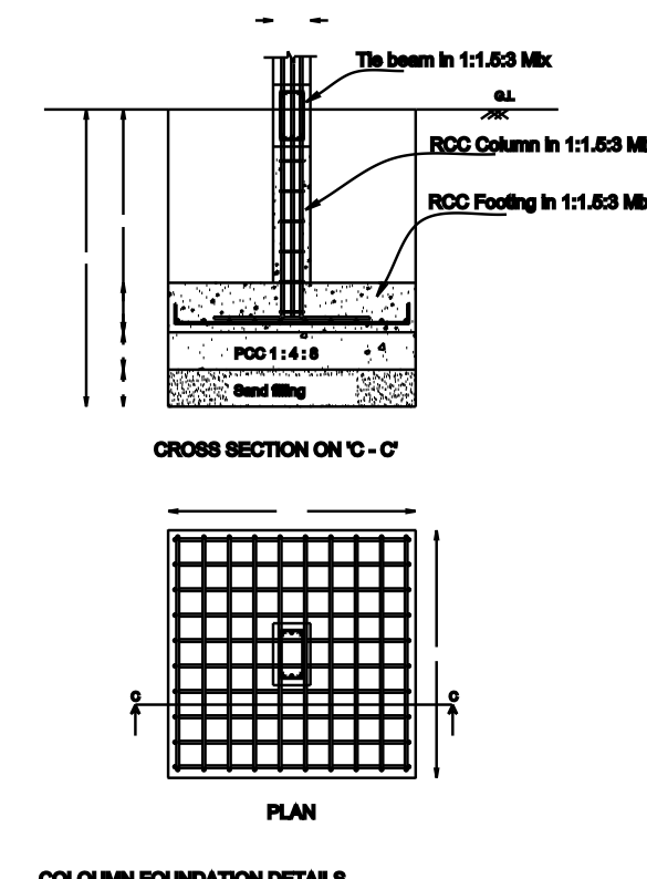
COLOUMN FOUNDATION DETAIL
