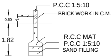
FOUNDATION DETAILS
