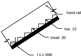
STAIR
