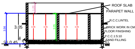
SECTION ON SS
