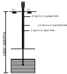
BORE WELL
