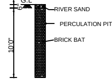
PERCOLATION PIT
