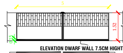
GATE ELEVATION
