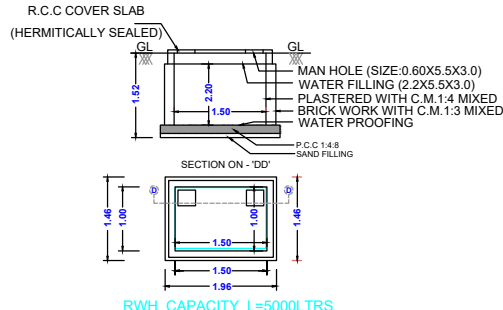
DETAILS OF COLLECTION SUMP FOR RAIN PLAN
