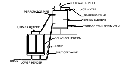
DETAILS OF SOLAR WATER HARVESTING (NTS)
