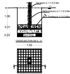
COLOUMN FOUNDATION
