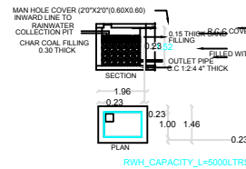
DETAILS OF RAINWATER HARVESTING
