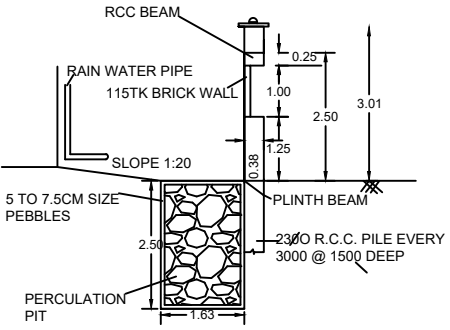
RAINWATER HARVESTING
