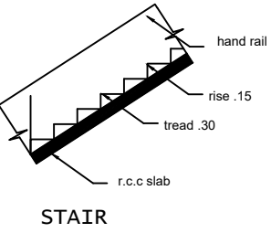
STAIR
