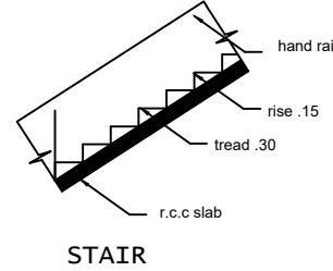
STAIR
