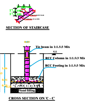
CROSS SECTION ON C - C
