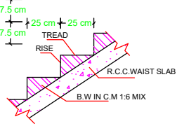
SECTION OF STAIRCASE
