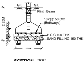
SCETION - 'XX'
