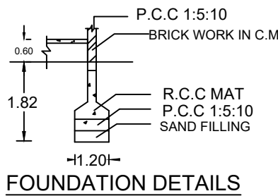
FOUNDATION DETAILS
