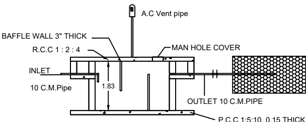
FRONT ELEVATION
